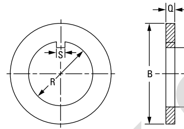
Fig. 54. Tongued washers.
