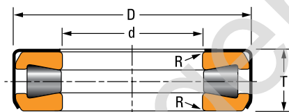
Fig. 83. Type TTC thrust tapered roller bearing assembly.
